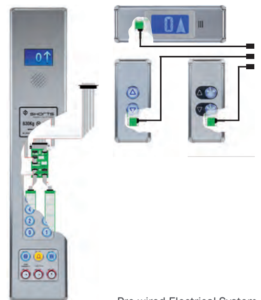
Pre-wired Electrical System
